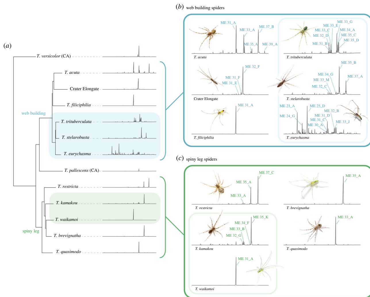
Figure 2. Representative chemical profiles of each species. (a) The GC-MS chromatograms of representative dragline extracts from females of each species positioned next to a reduced phylogenetic tree. The web building clade is indicated in the dark blue while the spiny leg clade is indicated in the dark green colour. The light blue and light green blocks highlight the closely related species that co-occur in both the web building and spiny leg clades respectively. (b) A closer look at the chromatograms of Hawaiian Tetragnatha spiders from the web-building clade arranged in the same order as the phylogenetic tree (from top left down to top right down). The most abundant methyl ethers are labelled with their specific shorthand code and the light blue box surrounds the closely related sympatric web building species that can be found in Upper Waikamoi. (c) The same as (b) but for spiders from the spiny leg clade. The most abundant methyl ethers are labelled with their specific shorthand code and the light green box surrounds the closely related sympatric spiny leg species that can be found in Upper Waikamoi.
